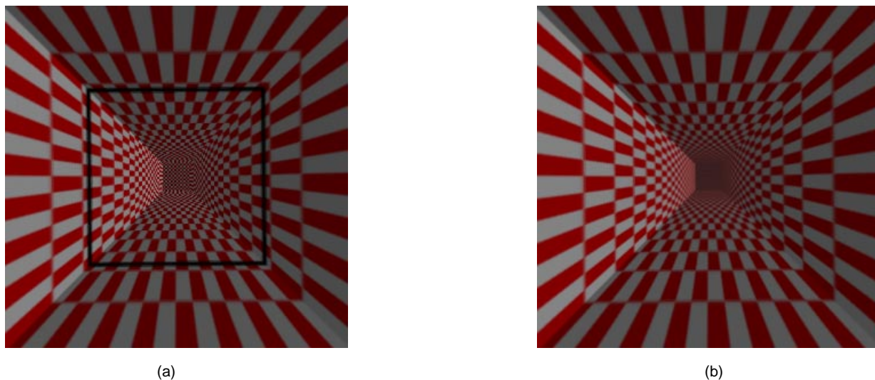
Fig. 5. Rendered image of a tunnel dataset with a checkerboard pattern. (a) Rendered with standard splatting; the black line is drawn at distance z_k . (b) Rendered with antialiased splatting.
