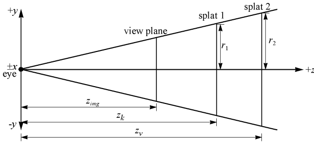
Fig. 3. The geometry for scaling the splats that are drawn beyond z_k .
