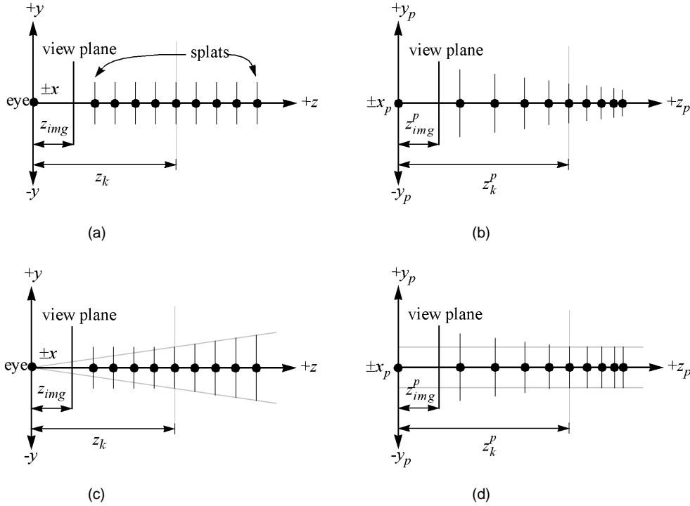
Fig. 2. A comparison of the standard splatting method ((a) and (b)) with our antialiased method ((c) and (d)). (a) The standard splatting method in eye space. (b) The standard splatting method in perspective space. (c) The antialiased splatting method in eye space. (d) The antialiased splatting method in perspective space.
