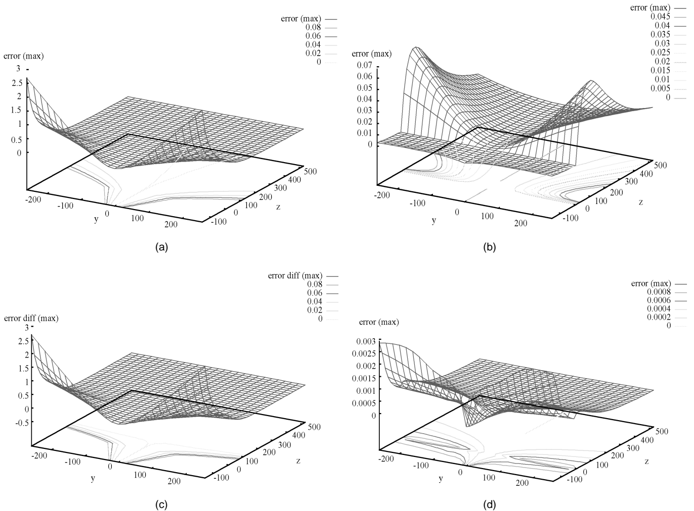
Fig. 10. Plots: (a) Maximum error for the grid-aligned kernel. (b) Maximum error for the practical ray-perpendicular kernel. (c) Difference of the maximum errors of the two kernel alignments (the iso-contours on the bottom planes denote lines of equal error). (d) Maximum error for the ideal kernel ray traversal when the trapezoidal stretching function is approximated by a box.
