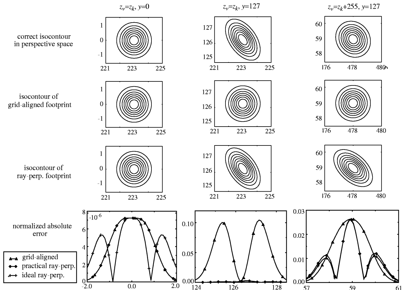
Fig. 9. The isocontours in the three top plots show the Gaussian kernel in perspective space. The bottom row shows how the errors of the ray integrals obtained by the approximate footprint methods of Fig. 8b (row 2) and Fig. 8c (row 3) compare with the correct ray integral of Fig. 8a (row 1). The absolute error is plotted, normalized by the maximum value of the ray integrals in the correct footprint. Column 1 is for voxels close to the eye and close to the viewing axis, column 2 is for voxels close to the eye, but far from the viewing axis, and column 3 is for voxel both far from the eye and far from the viewing axis.
