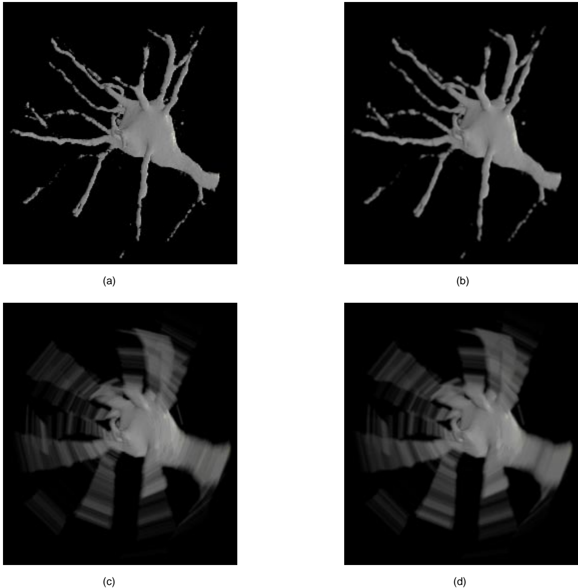
Fig. 12. Rendered image of a nerve dataset acquired from confocal microscopy. (a) Rendered with standard splatting. (b) Rendered with antialiased splatting. (c) Rendered with motion-blurred splats. (d) Rendered with antialiased, motion-blurred splats.
