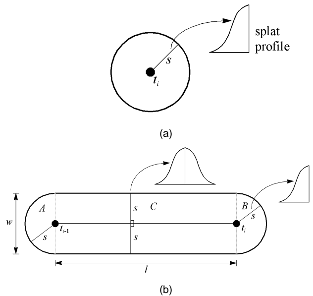
Fig. 11. The construction of a nonblurred and a motion-blurred splat. (a) A nonblurred splat (splat 1). (b) A motion-blurred splat (splat 2).
