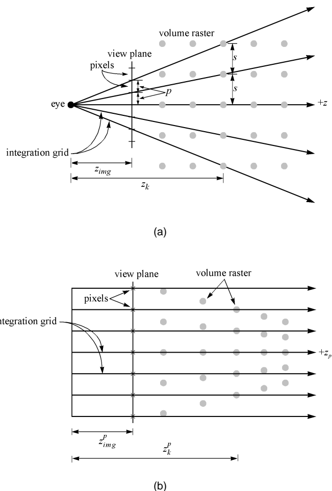
Fig. 1. Resampling the volume raster onto the integration grid. (a) In eye space. (b) In perspective space.
