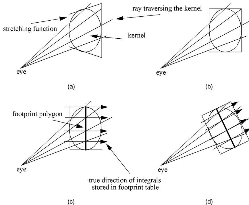
Fig. 8. Different stretchings of a rotationally symmetric kernel and possible placements of its footprint polygon in world space (2D case). (a) Trapezoidal kernel stretching. (b) Approximating the trapezoid of (a) with a box, the result is an elliptical kernel that is not rotationally symmetric. (c) Aligning the footprint polygon (thick line) with the volume grid, the result is that the indexed ray integrals do not correspond to the true ray integrals. (d) Aligning the footprint polygon orthogonally to the ray eye - (y_v, z_v) , which rectifies the problem of (c) in good approximation, however, also tilts the kernel stretching function.
