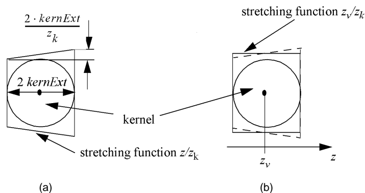
Fig. 7. (a) Stretching the splatting kernel according to the perspective stretching function z/z_k , which has the form of a trapezoid. (b) Stretching the kernel by the function z_v/z_k , which is a box.
