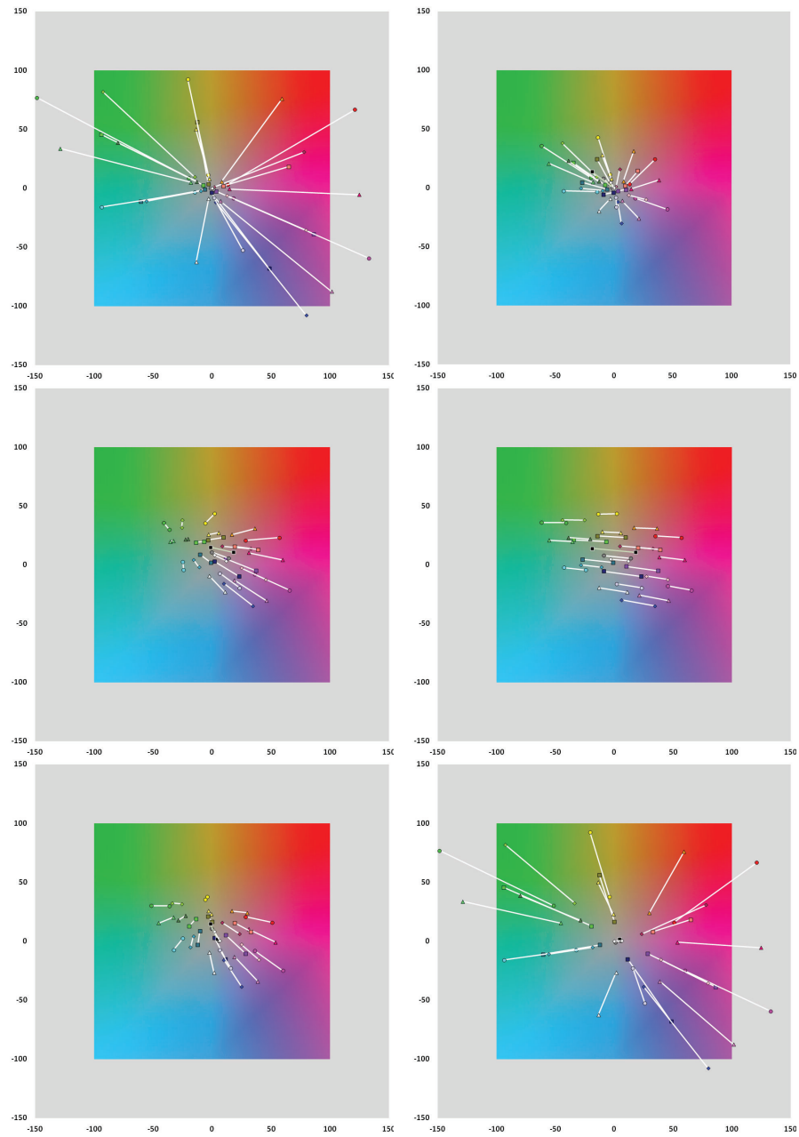
Fig. 1.7 Objective chromatic changes between textured backgrounds measured in [12], converted to CIELAB. Top left : no-background (outer) versus white background (inner). Top right : foliage background (outer) versus white background (inner). Center left : brick background (outer) versus sidewalk background (inner). Center right : brick background (right) versus foliage background (left). Bottom left : pavement background (outer) versus sidewalk background (inner). Bottom right : pavement background (inner) versus no background (outer).
