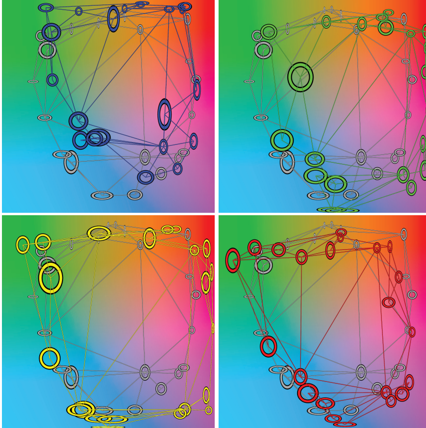
Fig. 1.8 The perceptual matching showed the color distortion in the nVisorST for four canonical chromatic backgrounds of solid color: Blue (upper left), Green (upper right), Yellow (lower left), and Red (lower right). Each graph is shown on CIELAB space and includes a gray reference grid of the matching as completed with no mediation by any AR display.
