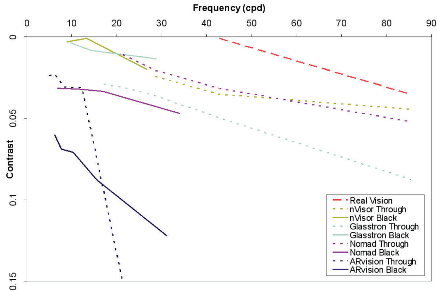
Fig. 1.4 The sampled CSF for four head-worn AR displays. The size of the target decreases as frequency (measured by cycles per degree) increases to the right. The contrast is typically graphed with lower contrast at the top of the vertical axis. In this test, the nVisorST performed well in both the see-through and graphical cases, the Glasstron provided sharp graphics, the Nomad provided clear see-through, while the ARvision struggled in both cases.
