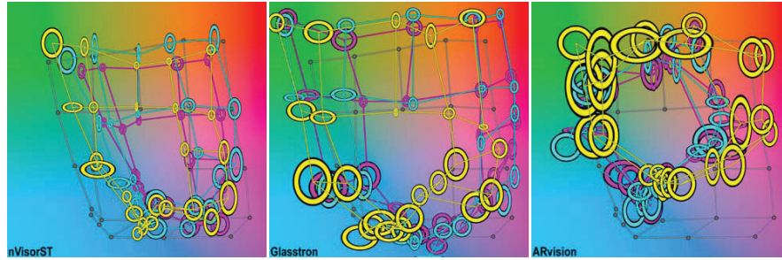
Fig. 1.6 The perceptual matching showed the color distortion in the nVisorST ( left ), Glasstron ( center ), and ARvision ( right ). The same three visual conditions are graphed with the same colors as in Figure 1.5. All data should be compared to the measured color gamut of the reference monitor, again mapped by the gray graph. In this figure and Figure 1.5, the CIELAB domain is represented by the L=65 slice with a and b in [-100,100] . This portion of the domain is also depicted in Figures 1.7 and 1.8 and thus may be used to help compare the data in all four graphs.
