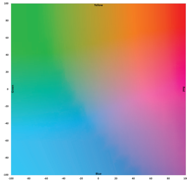
Fig. 1.3 The CIELAB space aimed to both mimic the physiological measurements of the eye and form a perceptually uniform color space. This slice at lightness L = 65 shows the a axis running from green at the left to red at the right and the b axis running from blue at the bottom to yellow at the top. The origin of the ab plane is the gray point in the center of this plot.
