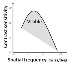
Fig. 1.1 The canonical shape of the contrast sensitivity function, graphed as a function of spatial frequency for size and contrast threshold for sensitivity.
